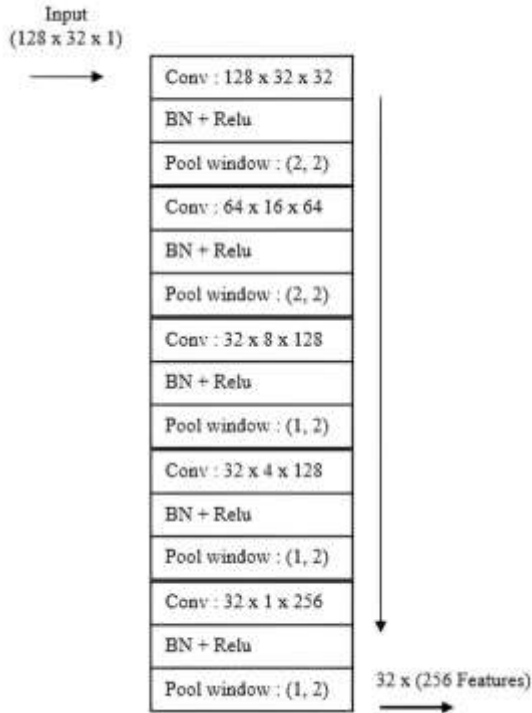
Fig 3. Architecture CNN Model
