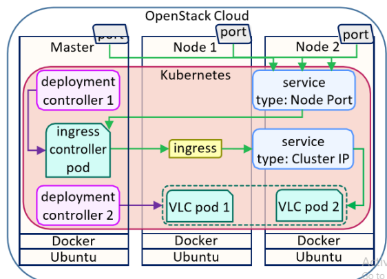
Fig. 7. Concrete architecture for deploying applications with Kubernetes – N-Way Active redundancy model
