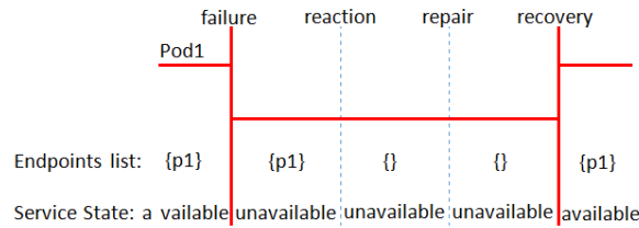
Fig. 6. Analysis of experiments with Kubernetes under the default configuration and No-Redundancy redundancy model – evaluating the repair actions.
