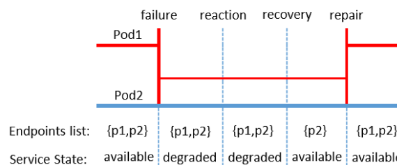
Fig. 8. Analysis of experiments with Kubernetes under the default configuration and N-Way Active Redundancy model – evaluating the impact of redundancy
