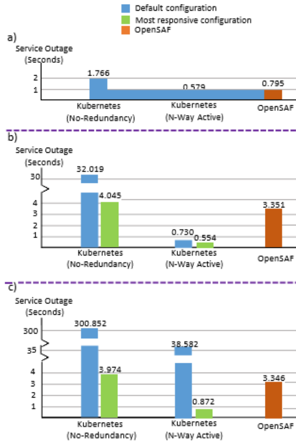
Fig. 9. Comparing Kubernetes and OpenSAF from availability perspective. a) VLC container failure scenario, b) Pod container failure scenario, c) Node failure scenario
